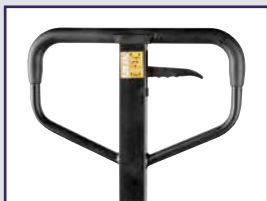
3-function hand control (raise, neutral and lower) and spring-loaded self-righting safety loop handle.
